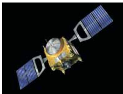
VenusExpress
